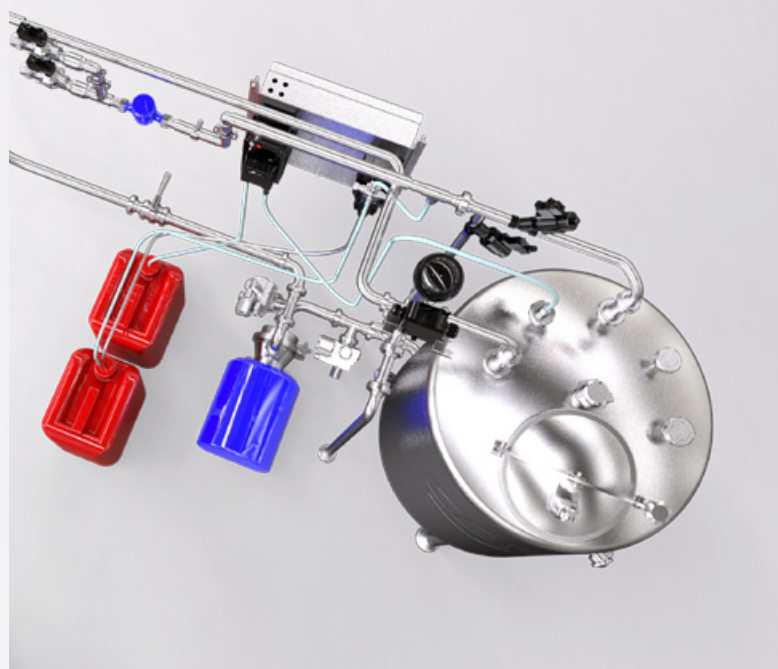
Detail: automated pumping system
