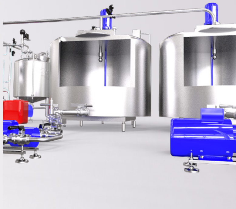
Detail: sprayball cleaning system
